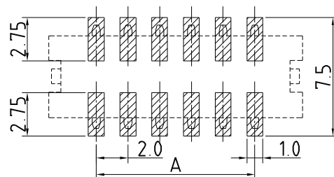
P.C.B LAYOUT Dimension and Order Information
