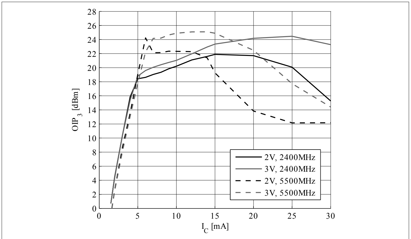
Figure 9 3rd order intercept point at output OIP_3 = f(I_C) , Z_S = Z_L = 50 \Omega , V_{CE} , f = parameter
