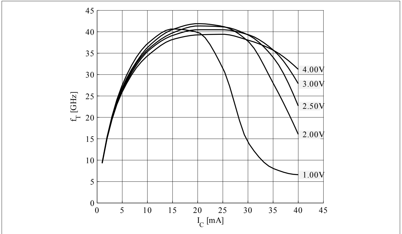
Figure 8 Transition frequency f_T = f(I_C) , f = 2 GHz, V_{CE} = parameter
