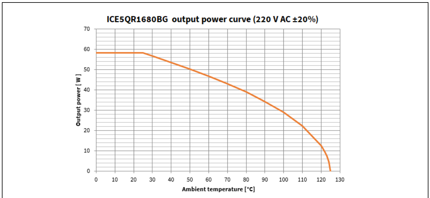
Figure 32 Output power curve of ICE5QR1680BG, V_{IN}=220 V_{AC} ; P_{Out}=f(T_a)
