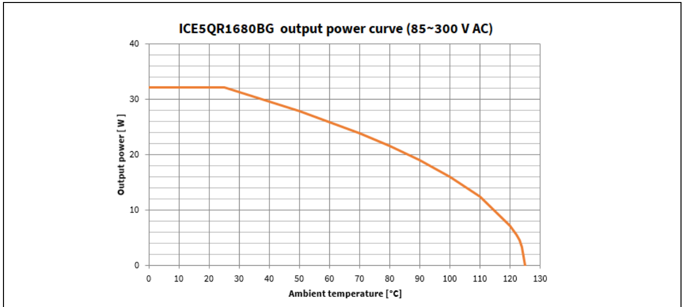
Figure 31 Output power curve of ICE5QR1680BG, V_{IN}=85\sim 300 V_{AC} ; P_{Out}=f(T_a)
