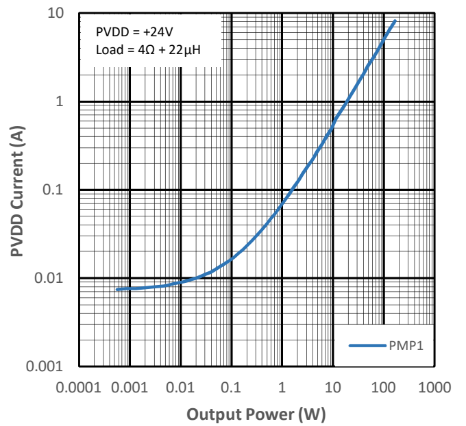
Figure 12-18 PVDD Current vs Output Power for PMP1
