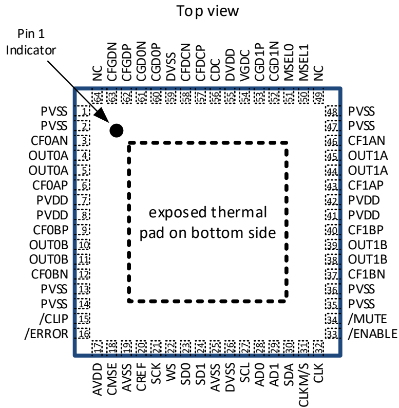
Figure 4-1 Pinout MA12070PQFN
