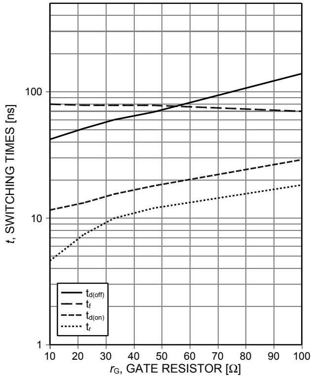
Figure 9. Typical switching times as a function of gate resistor (inductive load, T_{vj}=150^\circ\text{C} , V_{CE}=400\text{V} , V_{GE}=0/15\text{V} , I_C=5.0\text{A} , Dynamic test circuit in Figure E)
