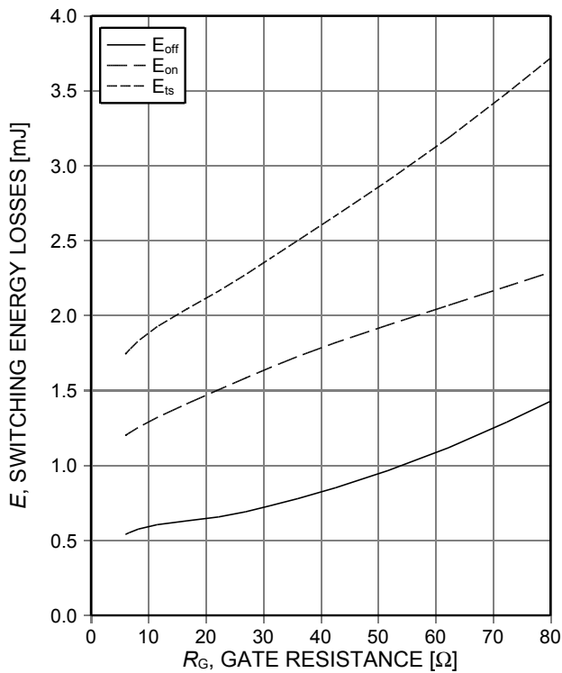
Figure 13. Typical switching energy losses as a function of gate resistance (inductive load, T_{vj}=175^\circ\text{C} , V_{CE}=400\text{V} , V_{GE}=0/15\text{V} , I_C=40\text{A} , dynamic test circuit in Figure E)
