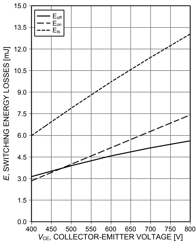
Figure 15. Typical switching energy losses as a function of collector emitter voltage (inductive load, T_{vj}=175^{\circ}\text{C} , V_{GE}=15/0\text{V} , I_C=40\text{A} , r_G=12\Omega , Dynamic test circuit in Figure E)
