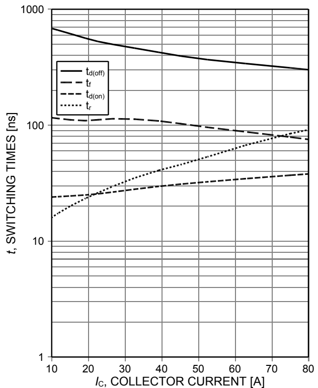
Figure 8. Typical switching times as a function of collector current (inductive load, T_{vj}=175^\circ\text{C} , V_{CE}=600\text{V} , V_{GE}=15/0\text{V} , r_G=12\Omega , Dynamic test circuit in Figure E)
