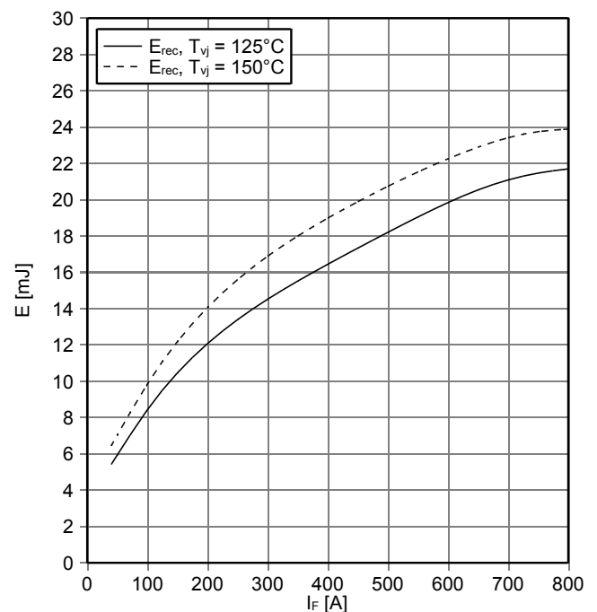
Schaltverluste Diode, D1 / D4 (typisch) switching losses Diode, D1 / D4 (typical) E_{rec} = f(I_F) R_{Gon} = 1.5\ \Omega , V_{CE} = 300\text{ V}
