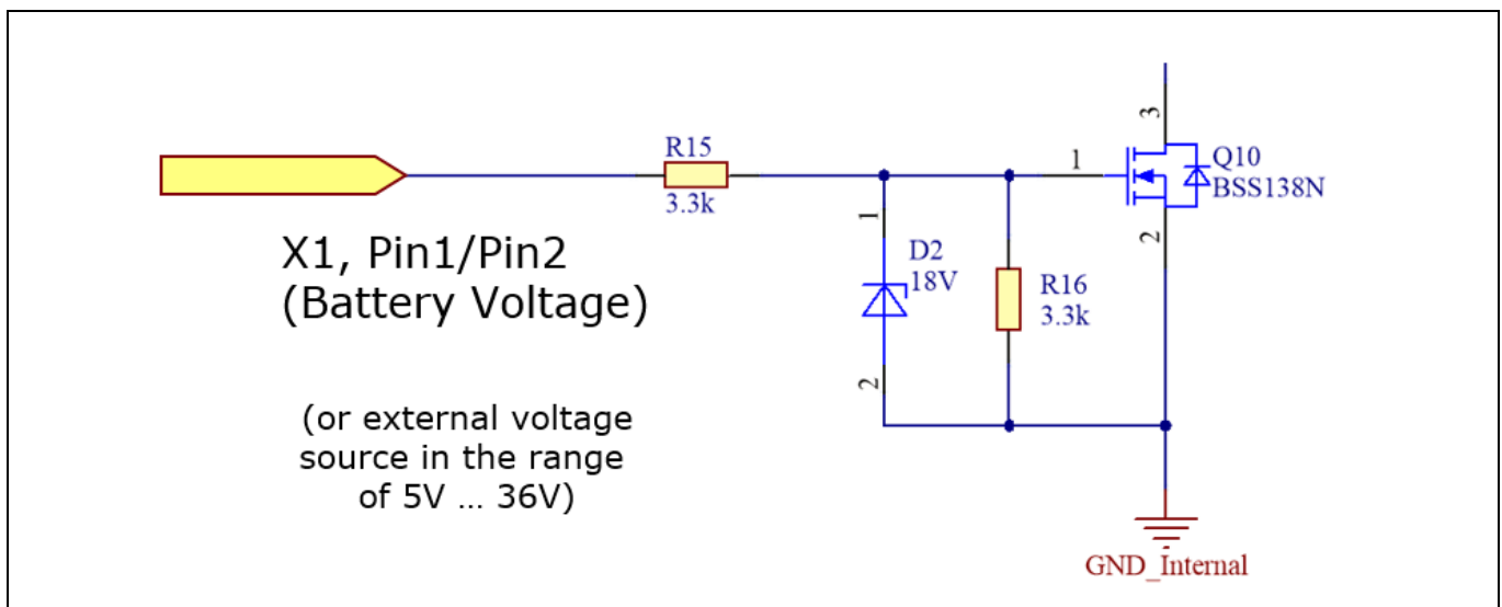
Figure 6 Input Stage
