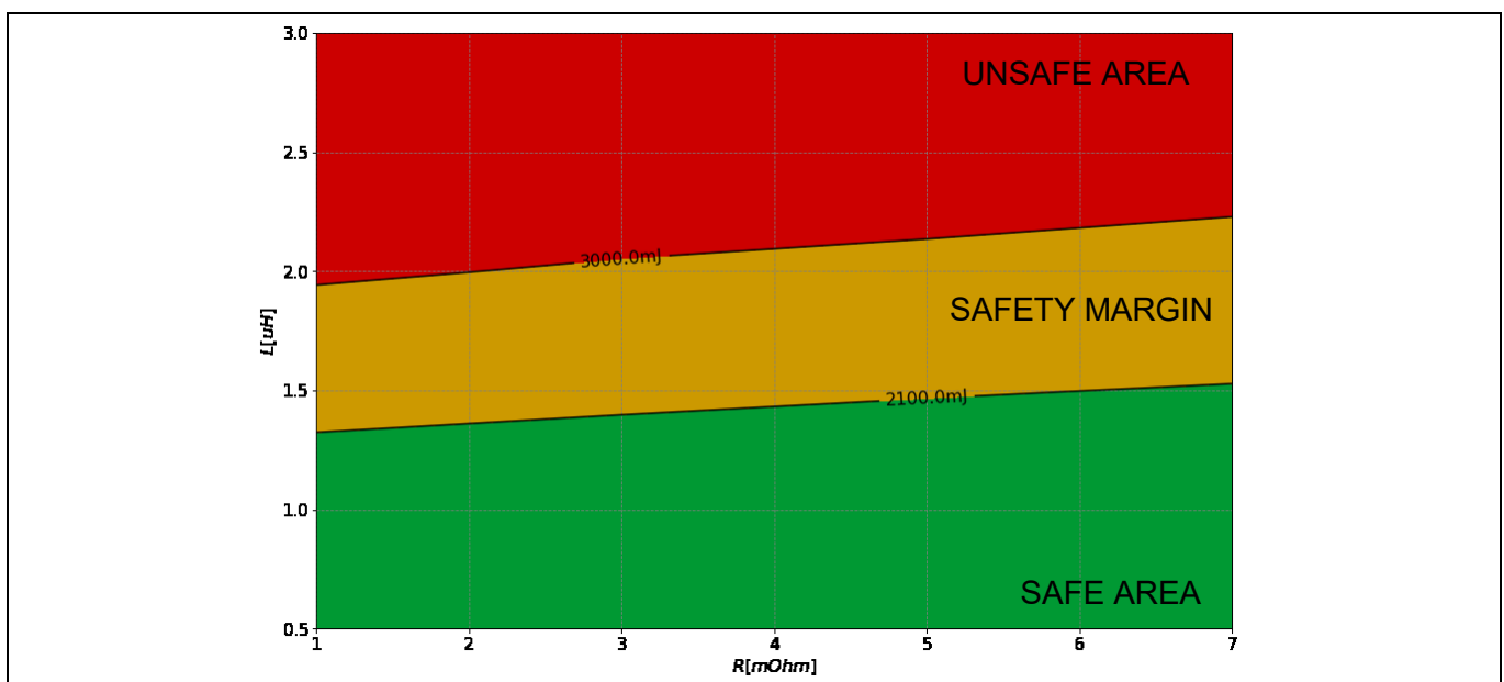
Figure 20 SOA for 12 V, Current = 1500 A, Limit = 6*500mJ, T j =25°C, limit extracted from Datasheet [2]
