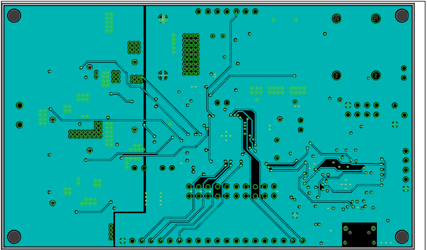
Figure 14 Layout Layer 3
