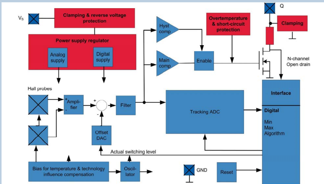
Block Diagram
