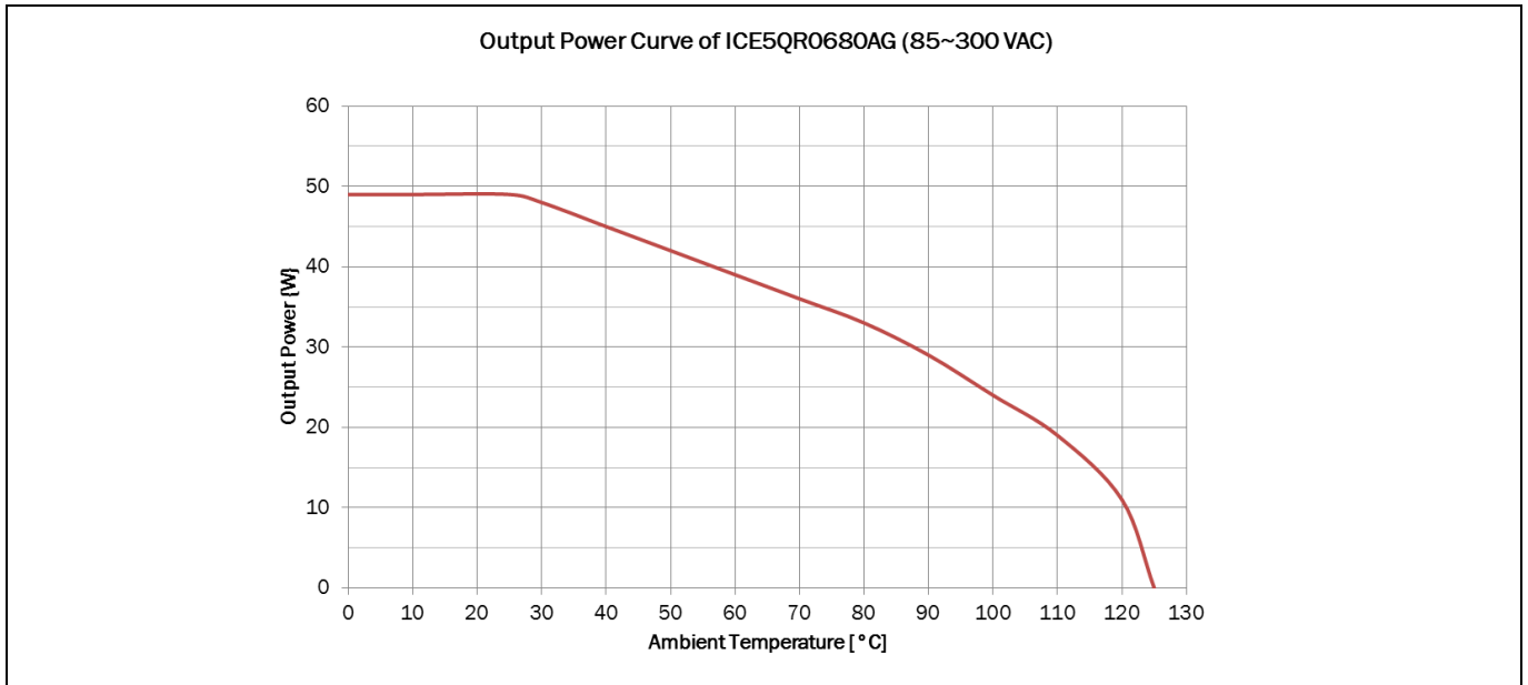
Figure 57 Output power curve of ICE5QR0680AG, V_{IN}=85\sim 300 V_{AC} ; P_{Out}=f(T_a)
