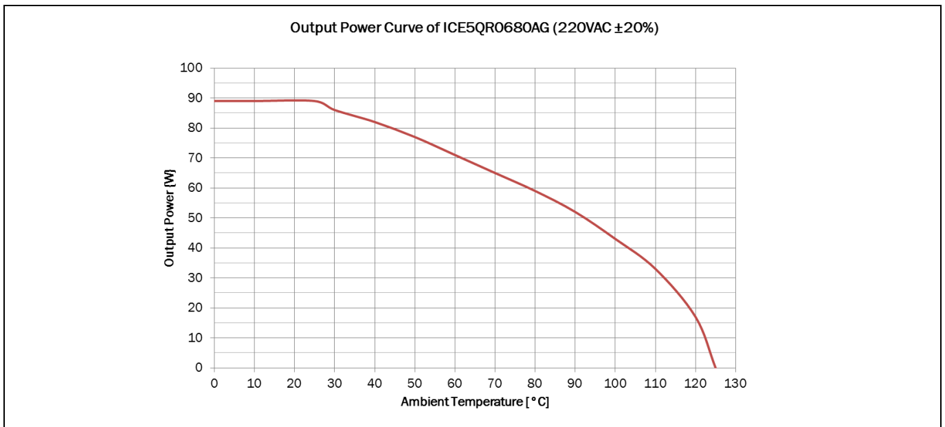
Figure 58 Output power curve of ICE5QR0680AG, V_{IN}=220 V_{AC} ; P_{Out}=f(T_a)
