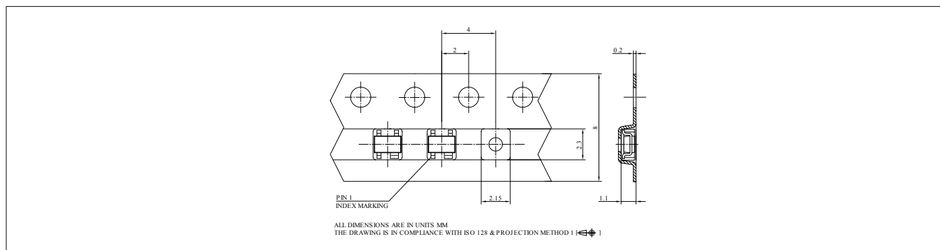
Figure 25 Tape dimensions
