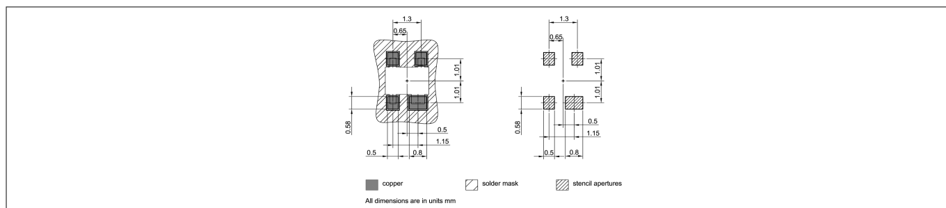
Figure 23 Foot print
