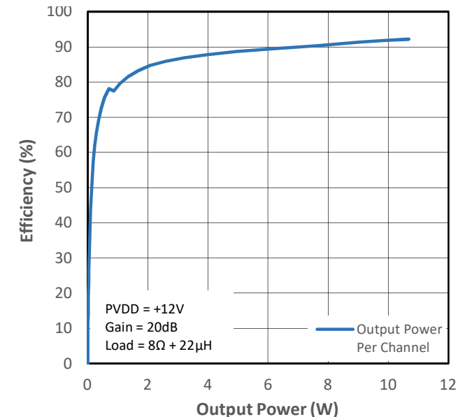
Figure 15-12 PMP4 Efficiency (VDD+PVDD) vs Output Power
