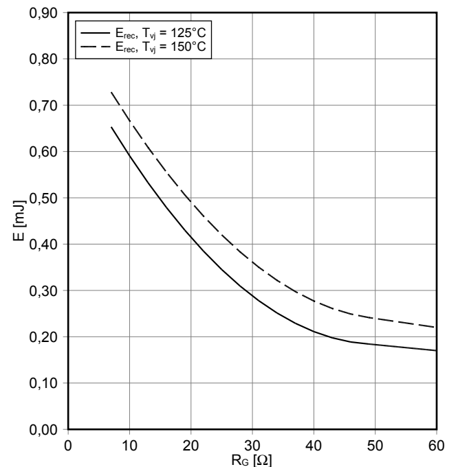
Schaltverluste Diode, D2 / D3 (typisch) switching losses Diode, D2 / D3 (typical) E_{rec} = f(R_G) I_F = 30 A , V_{CE} = 400 V
