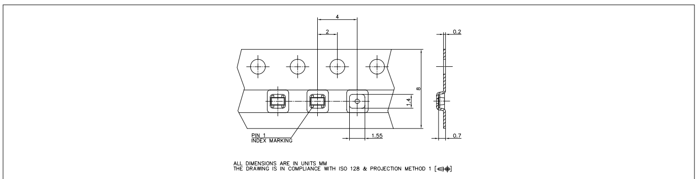
Figure 25 Tape dimensions
