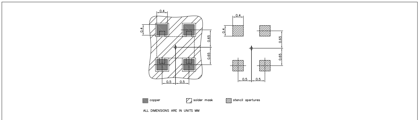
Figure 23 Foot print
