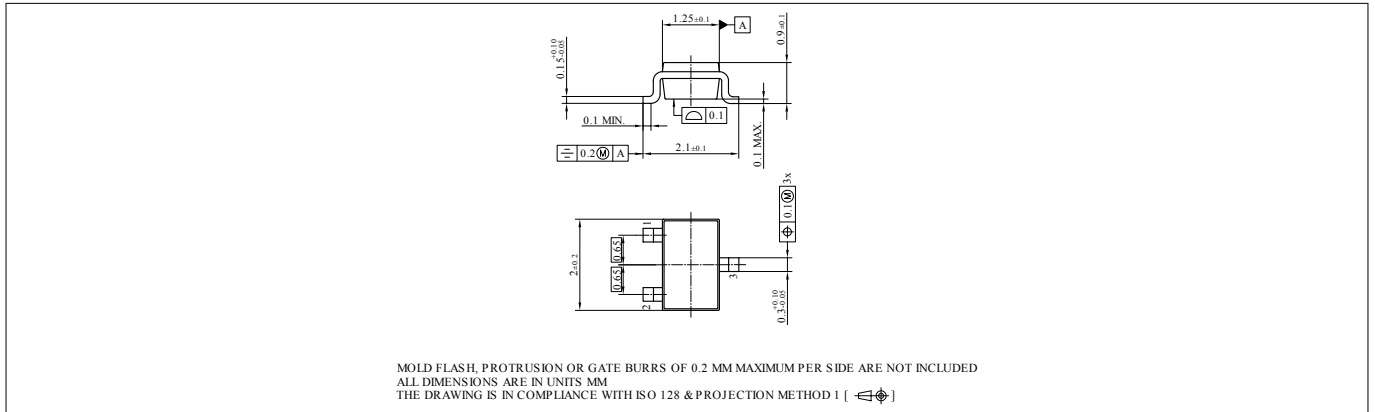
Figure 7 Package outline
