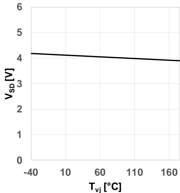
Figure 12 Typical body diode forward voltage as a function of junction temperature ( V_{SD} = f(T_{vj}) , V_{GS} = 0V , I_{SD} = 25A )
