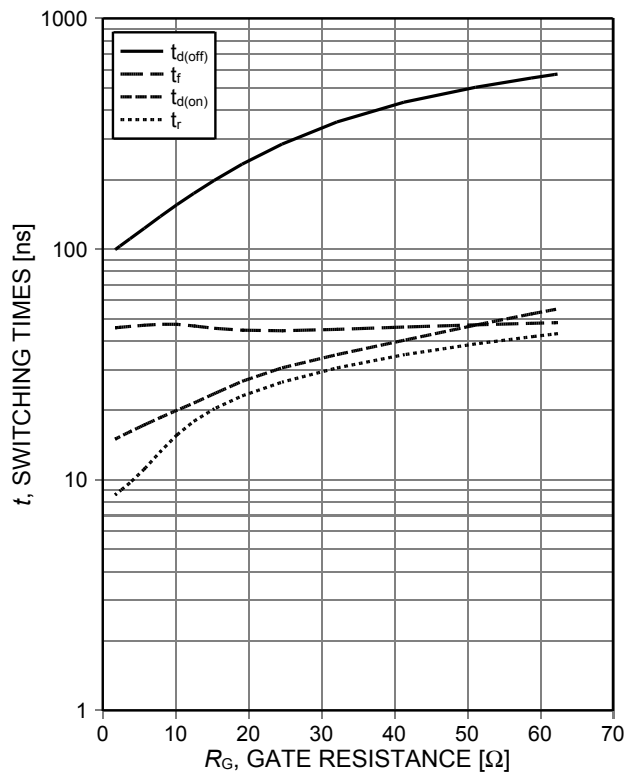
Figure 8. Typical switching times as a function of gate resistance (inductive load, T vj =150°C, V CE =400V, V GE =0/15V, I C =40A, dynamic test circuit in Figure E)
