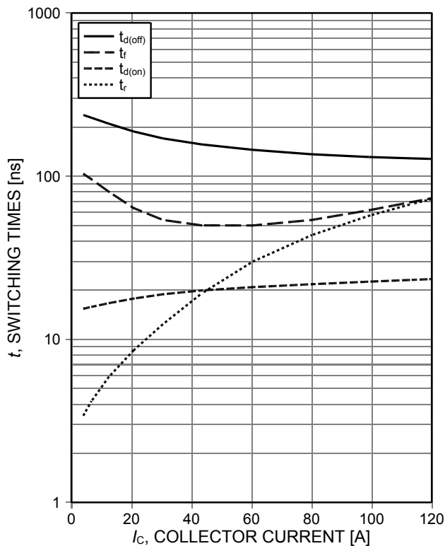
Figure 7. Typical switching times as a function of collector current (inductive load, T vj =150°C, V CE =400V, V GE =0/15V, R Gon =10Ω, R Goff =10Ω, dynamic test circuit in Figure E)
