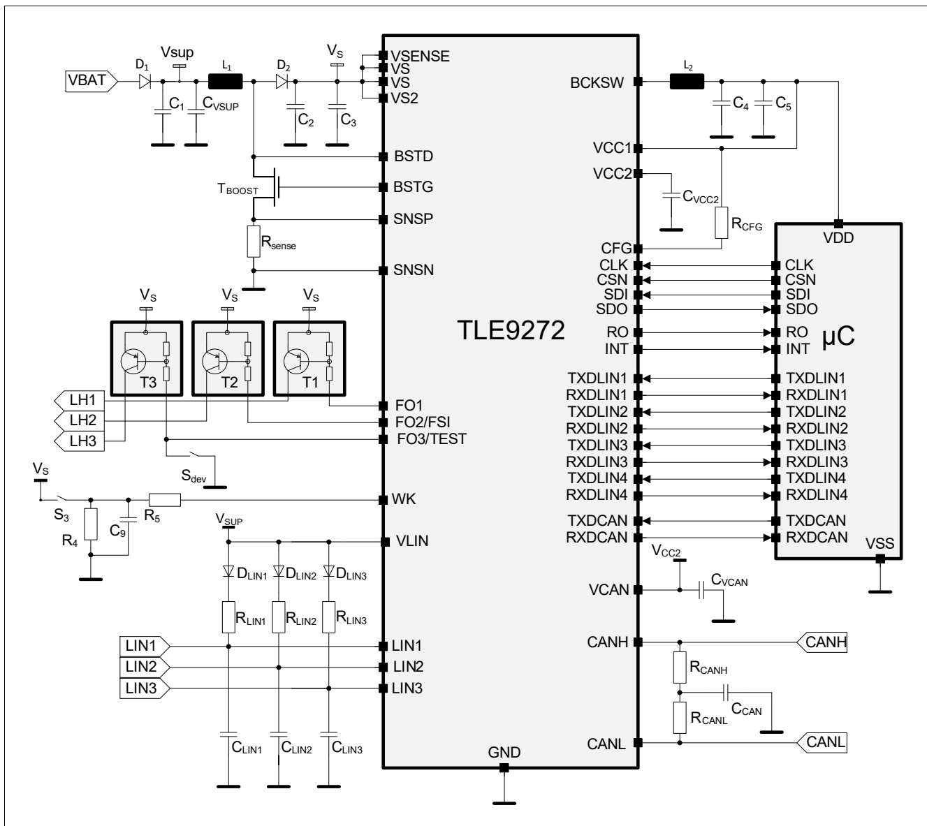
Figure 50 Application Diagram
