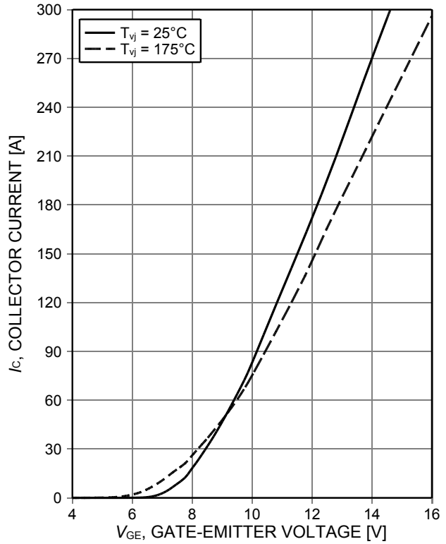
Figure 6. Typical transfer characteristic ( V_{CE}=20V )
