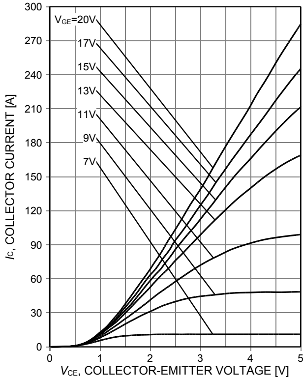
Figure 5. Typical output characteristic ( T_{vj}=175^{\circ}C )
