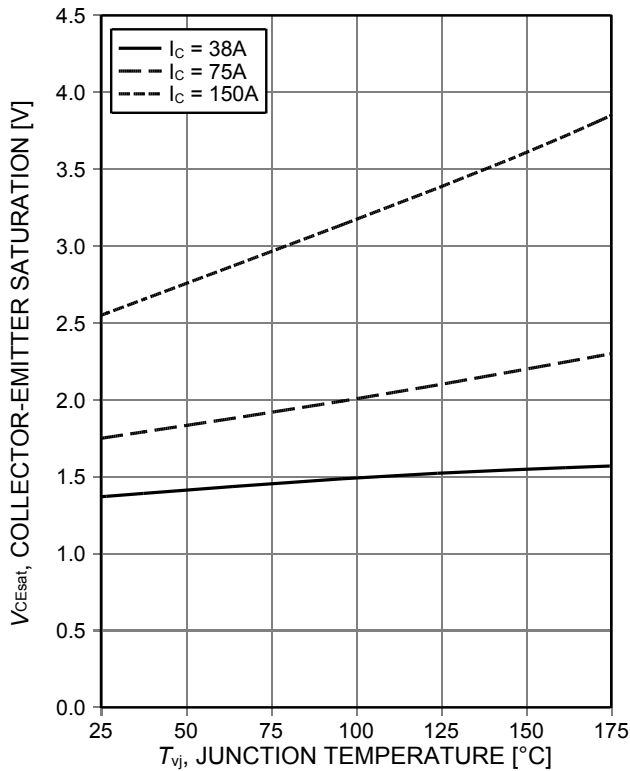
Figure 7. Typical collector-emitter saturation voltage as a function of junction temperature ( V_{GE}=15V )
