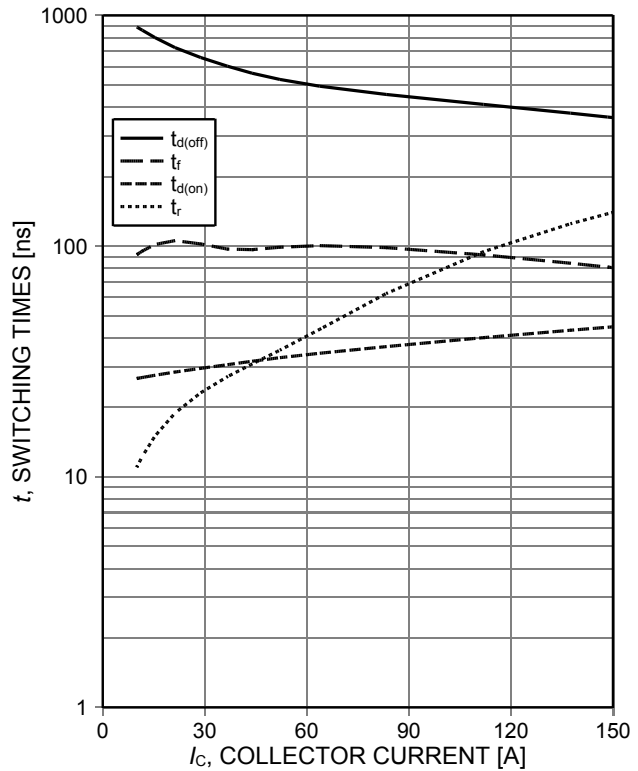
Figure 8. Typical switching times as a function of collector current (inductive load, T_{vj}=175^{\circ}C , V_{CE}=600V , V_{GE}=0/15V , r_G=6\Omega , Dynamic test circuit in Figure E)
