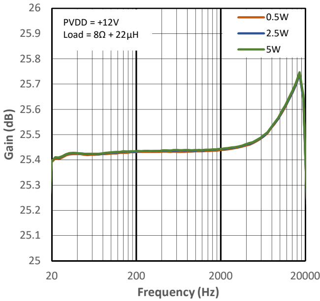
Figure 15-21 Gain vs Frequency for PMP0
