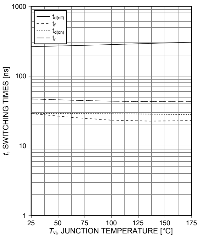
Figure 11. Typical switching times as a function of junction temperature (inductive load, V_{ce}=400\text{V} , V_{ge}=15/0\text{V} , I_c=100\text{A} , r_g=3.5\Omega , Dynamic test circuit in Figure E)
