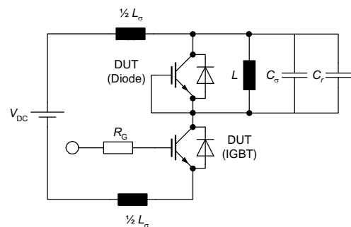
Figure E. Dynamic test circuit Leakage inductance L_{\sigma} = 180\text{nH} , Stray capacitor C_s = 40\text{pF} , Relief capacitor C_r = 4\text{nF} (only for ZVT switching)
