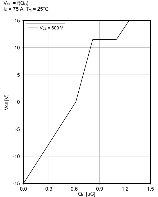
Gateladungs Charakteristik IGBT, Wechselrichter (typisch) gate charge characteristic IGBT, Inverter (typical) V_{GE} = f(Q_G) I_C = 75\text{ A} , T_{vj} = 25^\circ\text{C}
