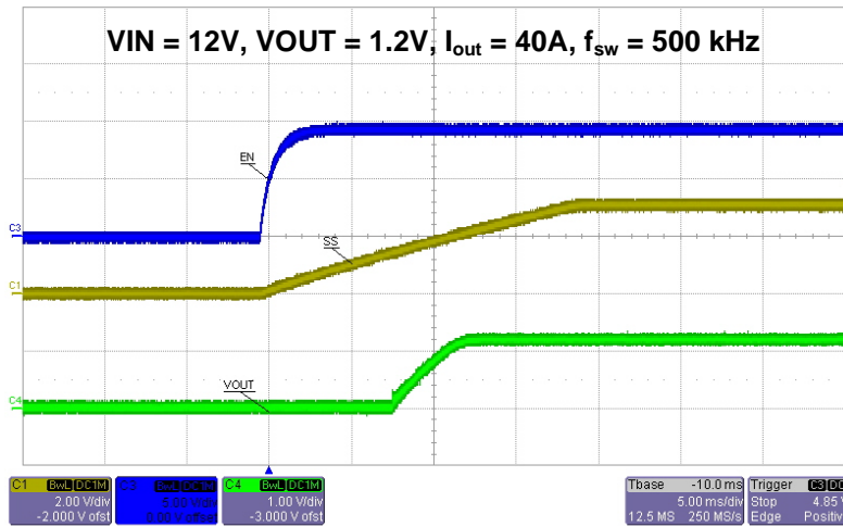
Fig. 5 Power Up Sequence (C3: EN, C1: SS1, C4: VOUT)
