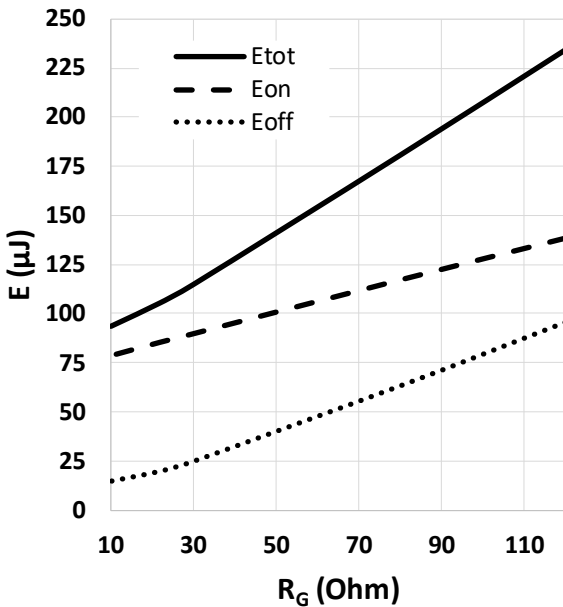
Figure 11 Typical switching energy losses as a function of gate resistance ( E = f(R_{G,ext}), V_{DD} = 1000V, V_{GS} = 0V/12V, I_D = 2A, T_{vj} = 175^\circ C , ind. load, test circuit in Fig. E, diode: body diode at V_{GS} = 0V )
