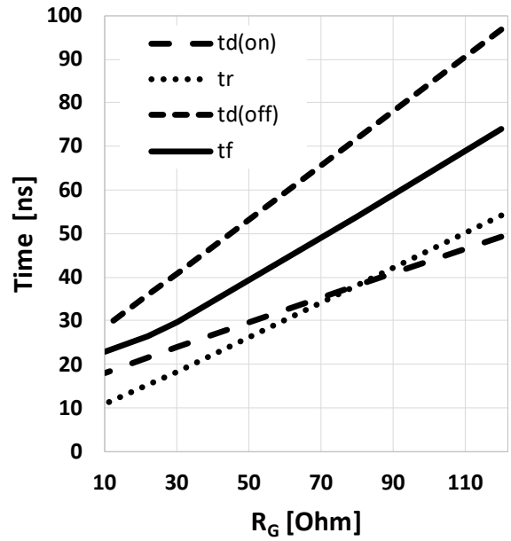
Figure 14 Typical switching times as a function of gate resistor (t = f(R_{G,ext}), V_{DD} = 1000V, V_{GS} = 0V/12V, I_D = 2A, T_{vj} = 175^\circ C, \text{ind. load, test circuit in Fig. E, diode: body diode at } V_{GS} = 0V)
