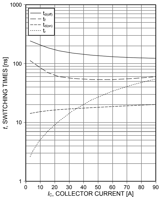
Figure 7. Typical switching times as a function of collector current (inductive load, T_{vj}=150^\circ\text{C} , V_{CE}=400\text{V} , V_{GE}=0/15\text{V} , R_{Gon}=13\Omega , R_{Goff}=13\Omega , dynamic test circuit in Figure E)
