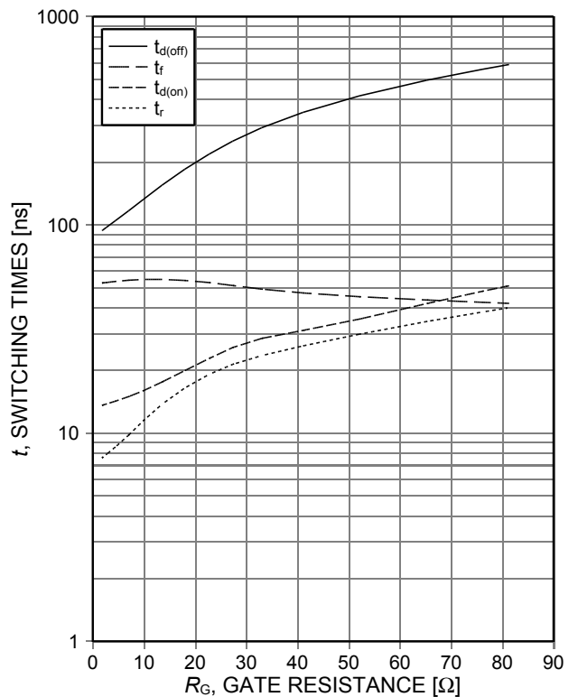
Figure 8. Typical switching times as a function of gate resistance (inductive load, T_{vj}=150^\circ\text{C} , V_{CE}=400\text{V} , V_{GE}=0/15\text{V} , I_c=30\text{A} , dynamic test circuit in Figure E)
