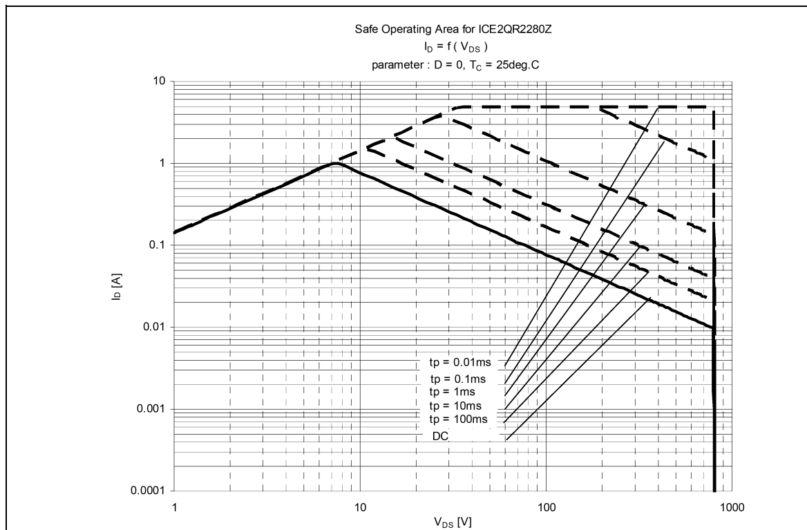
Figure 10 Safe Operating Area(SOA) for ICE2QR2280Z
