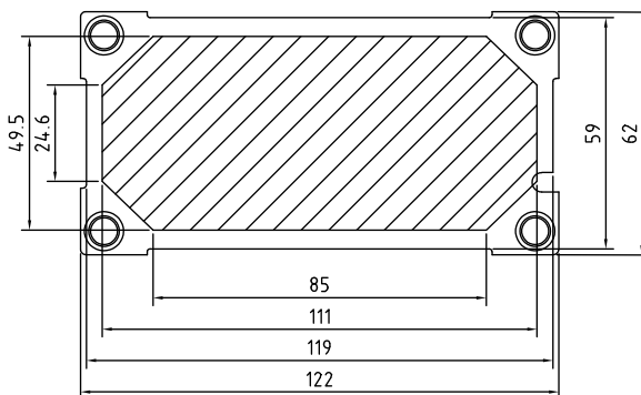
restricted area for Thermal Interface Material
