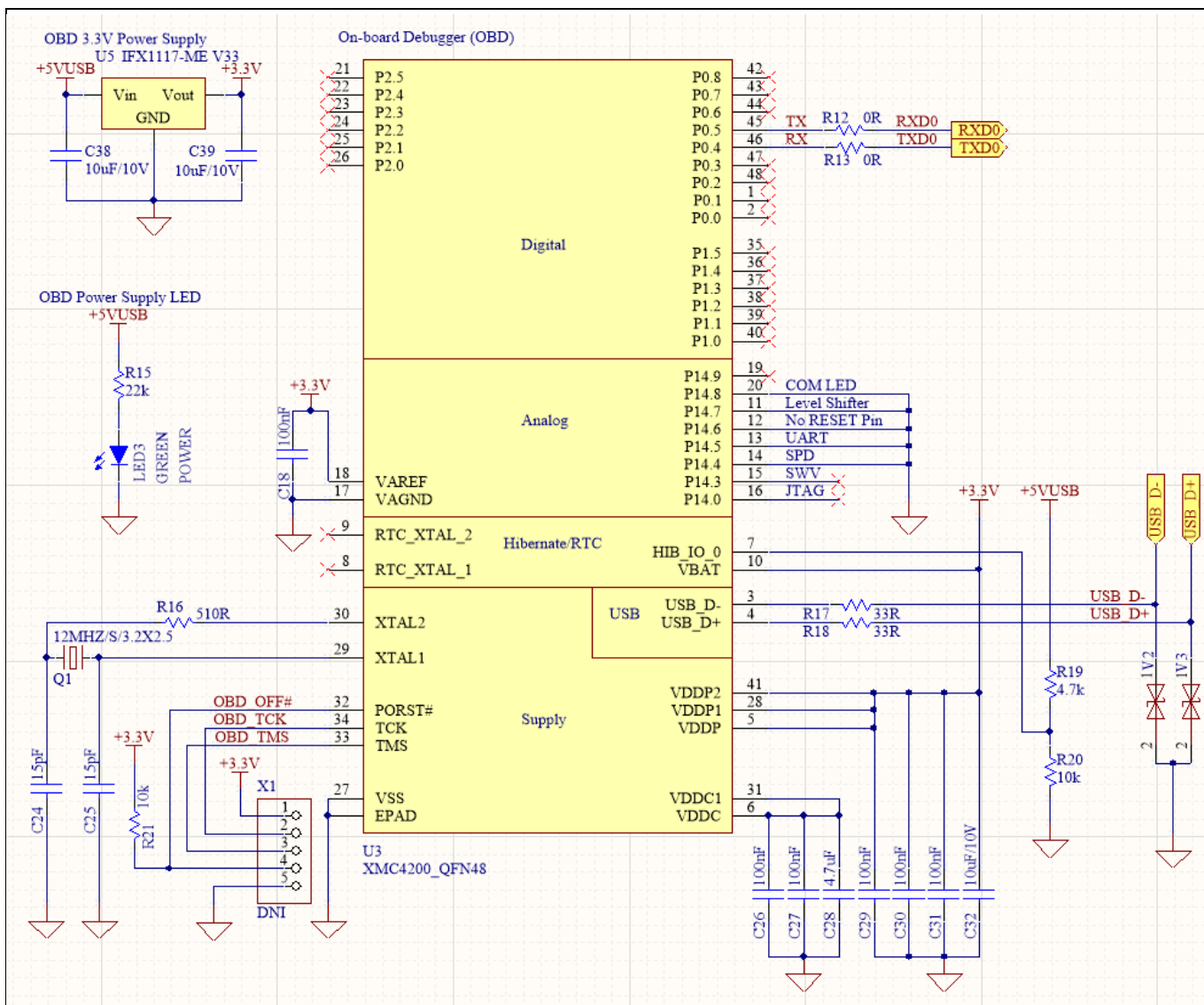
Figure 4 On-board debugger
