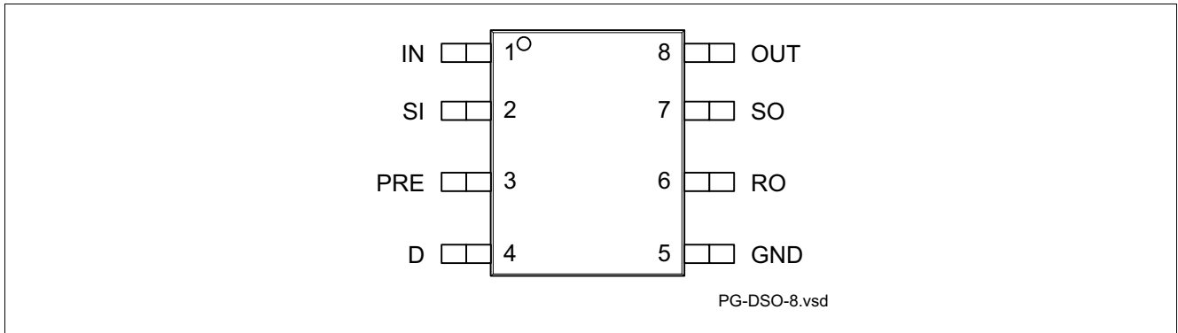
Figure 2 Pin Configuration PG-DSO-8
