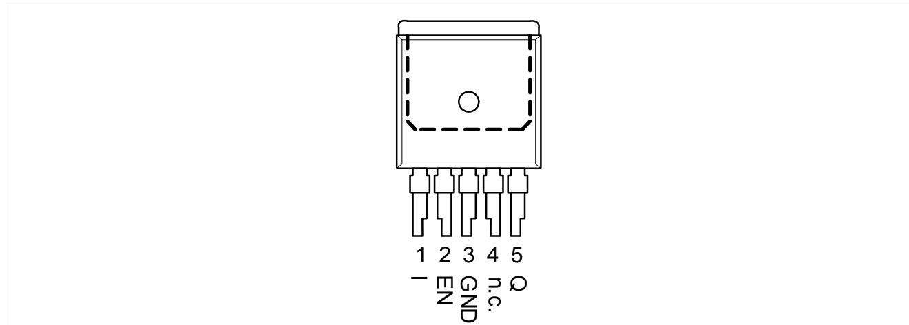
Figure 2 Pin configuration
