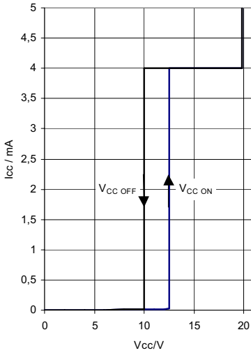
I_{CC} versus V_{CC}
