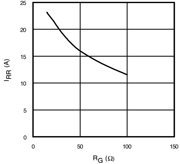
Fig. 18 - Typical Diode I RR vs. R G T J = 150°C; I F = 10A
