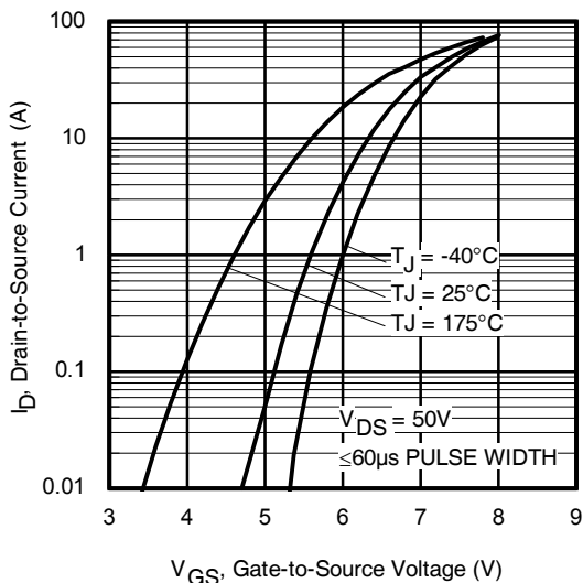
Fig 5. Transfer Characteristics
