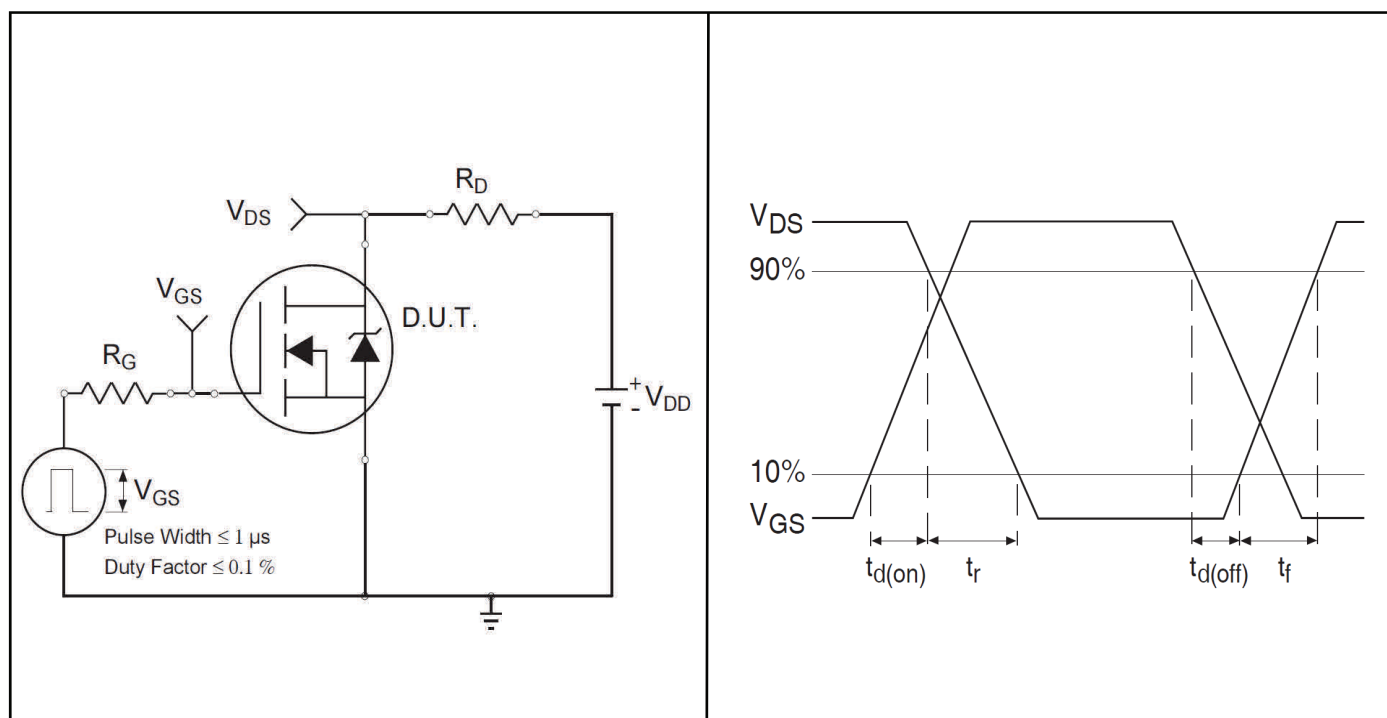
Figure 19b Switching Time Waveforms
