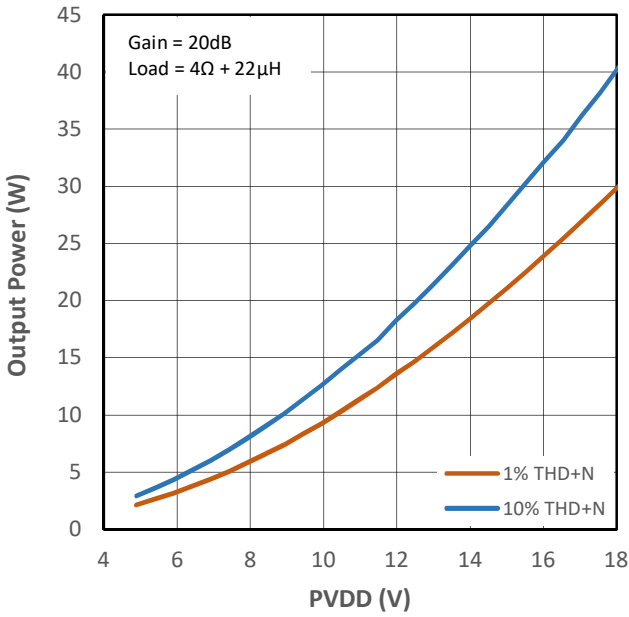
Figure 10-21 Output Power vs PVDD Voltage for PMP0
