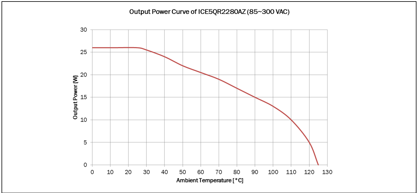
Figure 47 Output power curve of ICE5QR2280AZ, V_{IN}=85\sim 300 V_{AC} ; P_{Out}=f(T_a)
