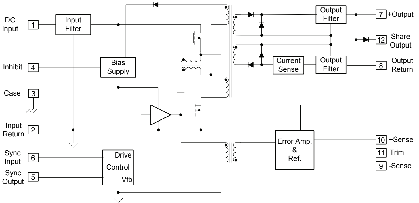
Fig 11 . Block Diagram
