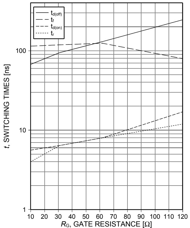
Figure 8. Typical switching times as a function of gate resistance (inductive load, T vj =175°C, V CE =400V, V GE =0/15V, I c =2,5A, dynamic test circuit in Figure E)
