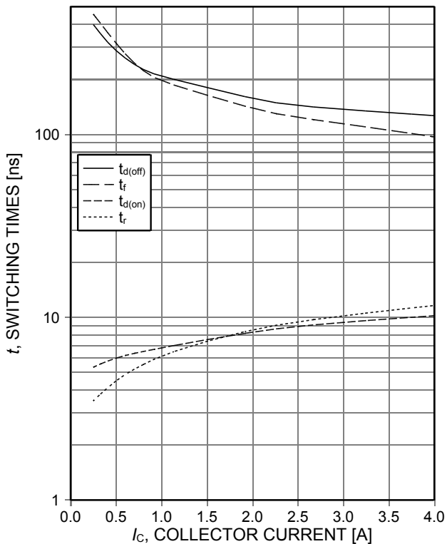
Figure 7. Typical switching times as a function of collector current (inductive load, T vj =175°C, V CE =400V, V GE =0/15V, R Gon =68Ω, R Goff =68Ω, dynamic test circuit in Figure E)
