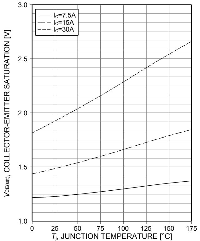
Figure 8. Typical collector-emitter saturation voltage as a function of junction temperature ( V_{\text{GE}}=15\text{V} )
