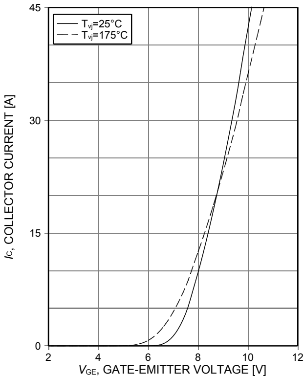
Figure 7. Typical transfer characteristic ( V_{\text{CE}}=20\text{V} )
