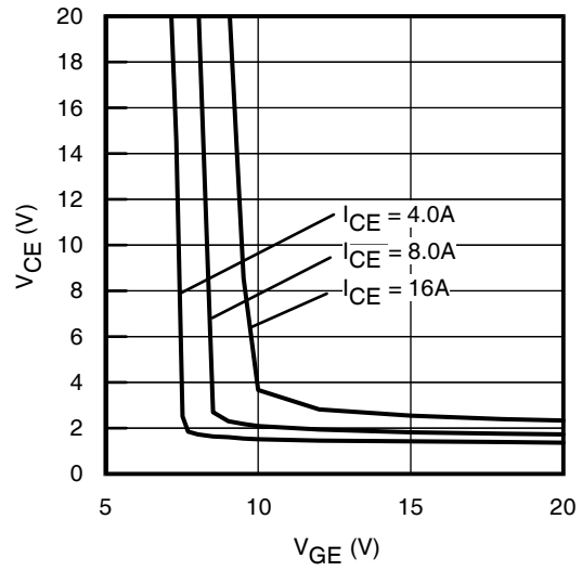
Fig. 9 - Typical V_{CE} vs. V_{GE} T_J = 25^\circ\text{C}
