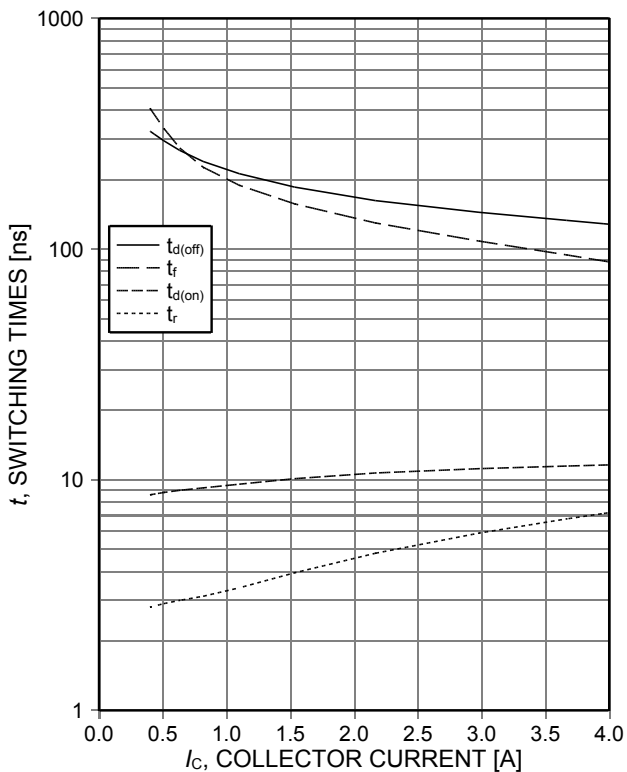
Figure 7. Typical switching times as a function of collector current (inductive load, T vj =175°C, V CE =400V, V GE =15/0V, r G =43Ω, Dynamic test circuit in Figure E)
