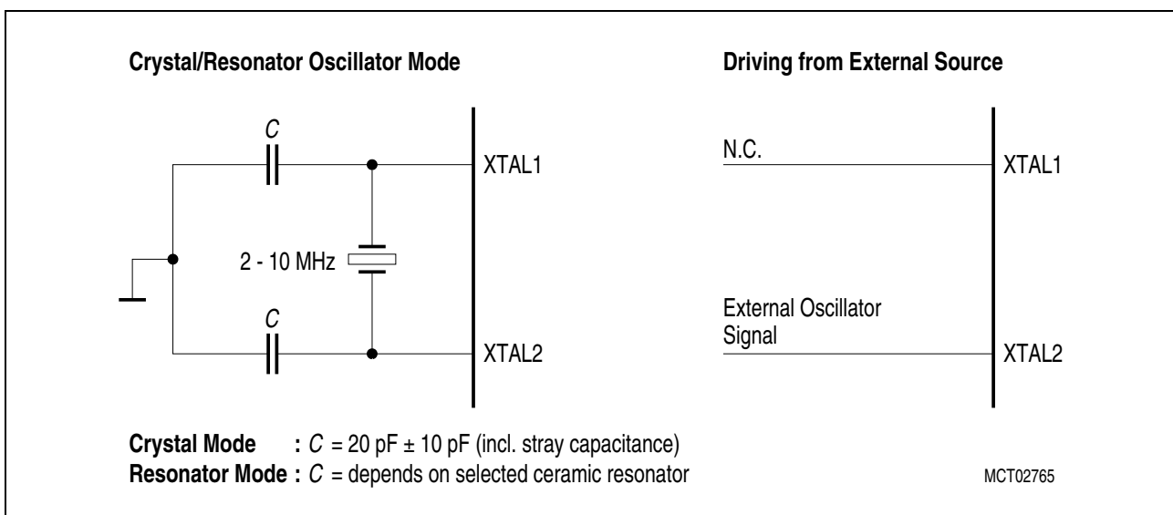
Figure 43 Recommended Oscillator Circuits for Crystal Oscillator
