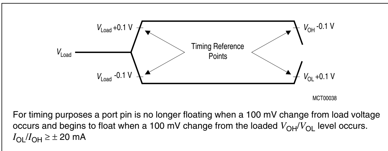
Figure 42 AC Testing: Float Waveforms
