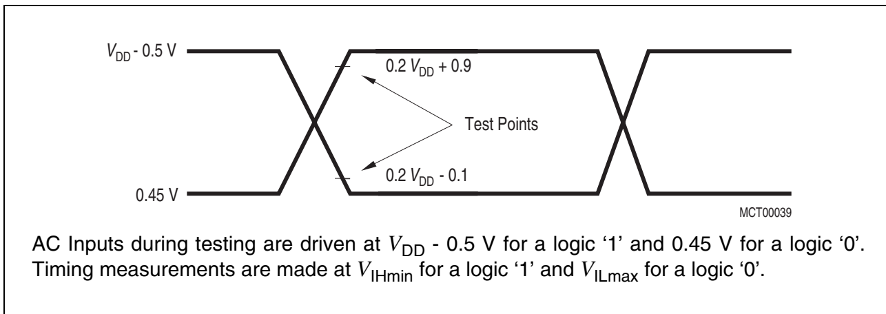
Figure 41 AC Testing: Input, Output Waveforms
