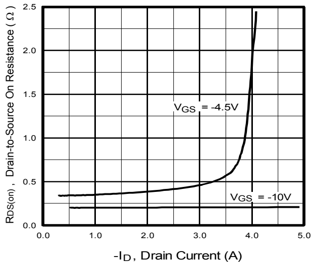
Fig 17. Typical On-Resistance Vs. Drain Current
