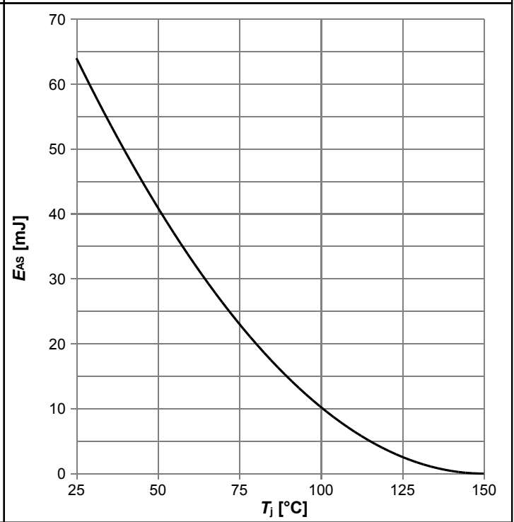
Diagram 12: Avalanche energy
