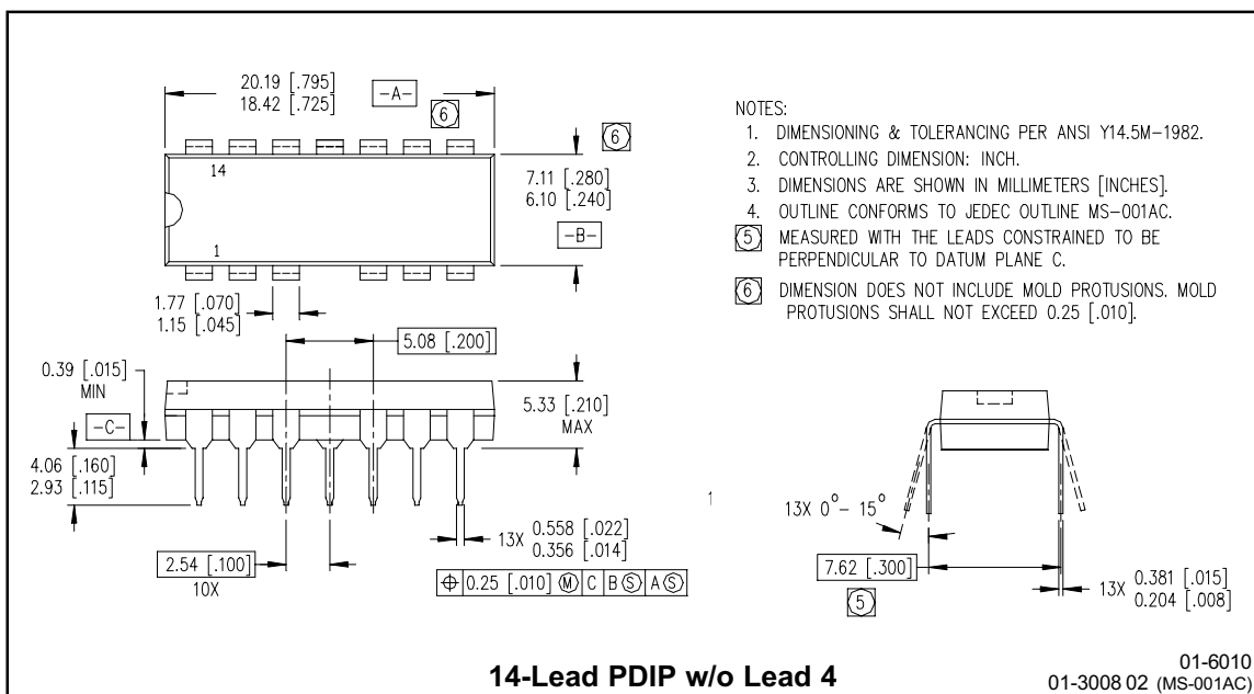
14-Lead PDIP
