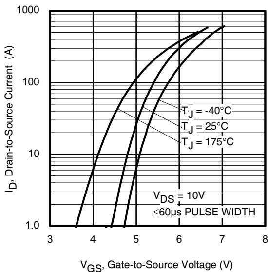
Fig 5. Transfer Characteristics
