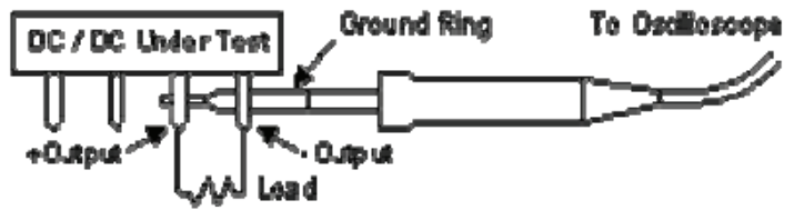
Figure 6. correct method to use the oscilloscope probe.
